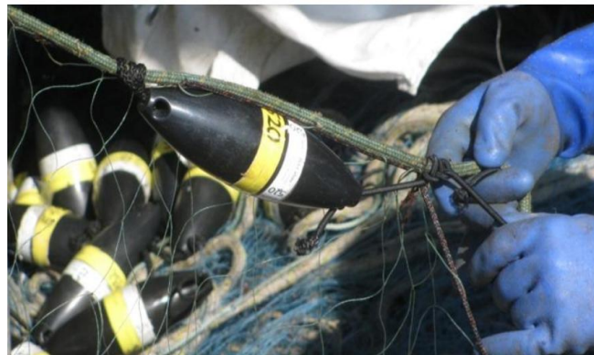
Fig. 4: “PAL” v.1 on the floatline of a gillnet
