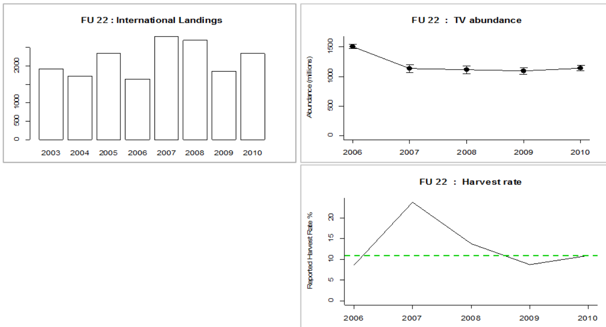
Figure 5.4.34.6.2 Nephrops in the Celtic Sea (FU 22). Recent international landings in tonnes for FU22 (Smalls) (top left); UWTV survey abundance for FU 22 (top right, proxy for SSB), and harvest rate (green dashed line represents F_{MSY} harvest ratio) (bottom right).
