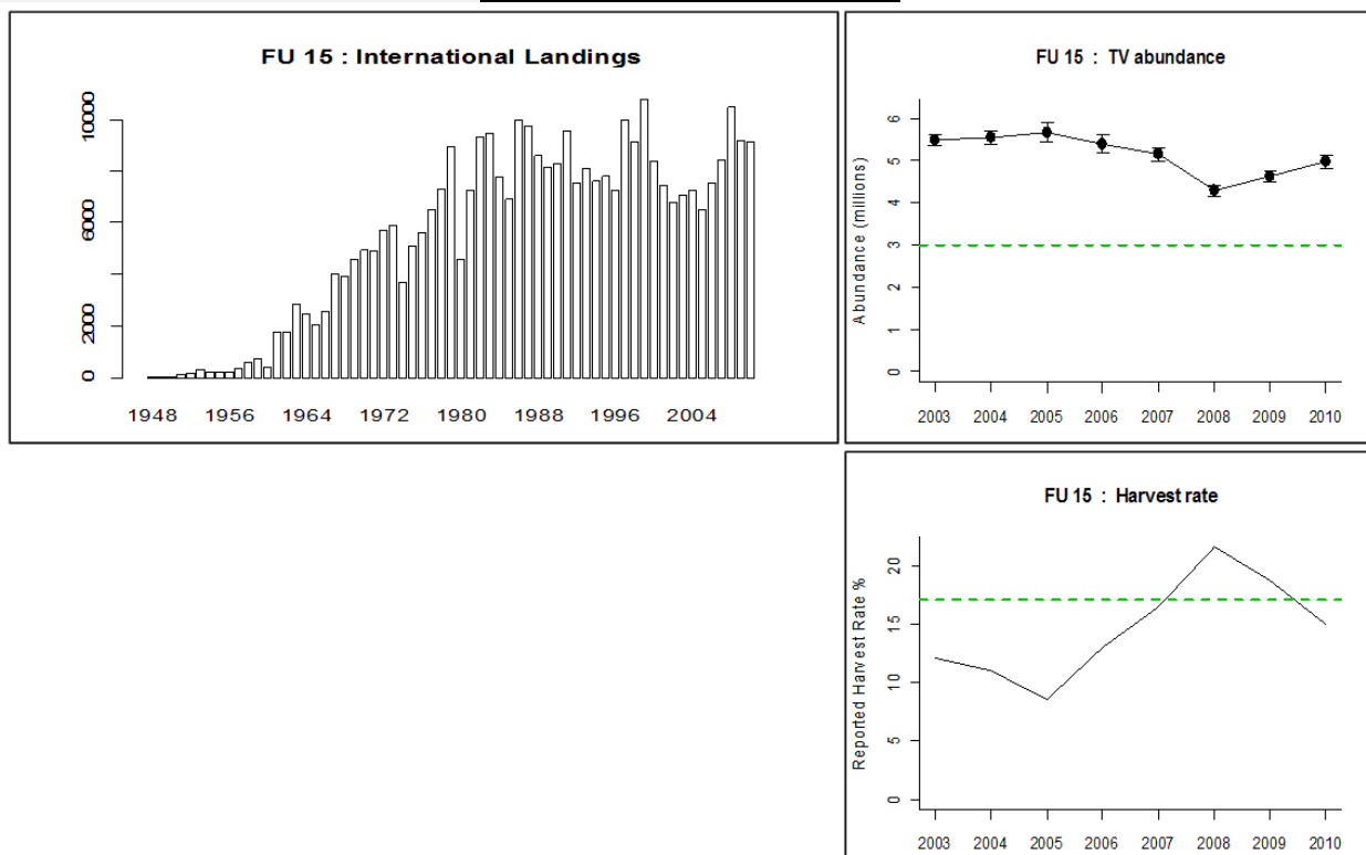
Figure 5.4.34.1 Nephrops in Irish Sea West (FU 15). Long-term trends in landings (tonnes), recent UWTV abundance (in millions; SSB proxy) (with scaled trawl survey cpue) and harvest rates (prior to 2007 the harvest rate is considered to be a minimum estimate due to possible under-reporting of landings). The horizontal lines represent MSY B_{trigger} (upper panel) F_{MSY} (lower panel).
