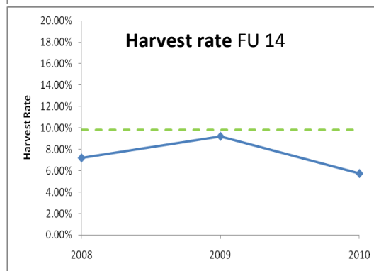
Figure 5.4.34.1.1 Nephrops , Irish Sea East (FU14): Long-term trends in landings (in tonnes), UWTV survey abundance with 95% confidence limits (in millions; SSB proxy) and harvest rate (green dashed line is F_{MSY} proxy).
