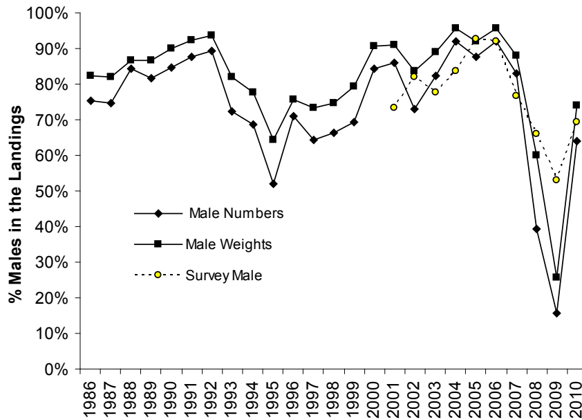
Figure 5.4.34.3.5 Nephrops on Porcupine Bank (FU 16). Sex ratio of landings and survey (SpPGFS-WIBTS-Q4) catches.
