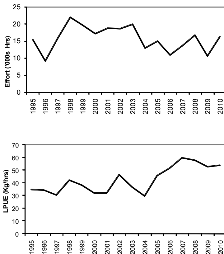
Figure 5.4.34.4.2 Nephrops in Aran Grounds (FU 17). Irish effort and lpue for Nephrops -directed fleet.
