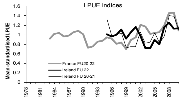
Figure 5.4.34.6.1 Nephrops in the Celtic Sea (FU 20–22). Long-term trends landings (t) for the whole area and from FU 22 since 1999 (grey bars) (top left). Nephrops directed fishing effort by country and total Nephrops directed effort (top right). Mean standardised lpue indices for Ireland FU 22 and FU 20-21 and France for FU 20-22 (mainly operating in FU20-21 during the last decade) (bottom right).
